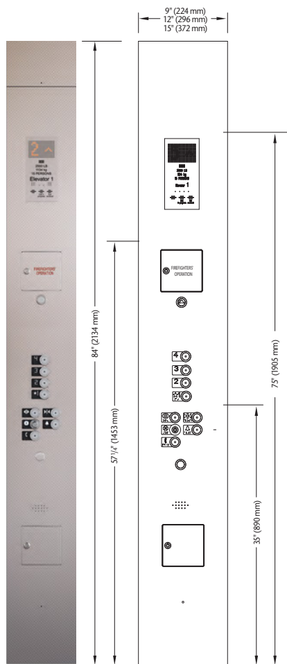
Car Operating Panel KSS 140
