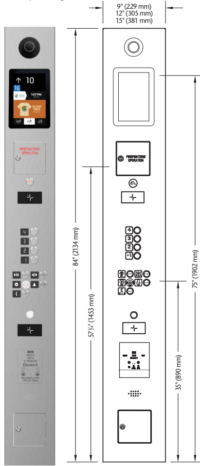
Emergency Video Communications Car Operating Panel*
