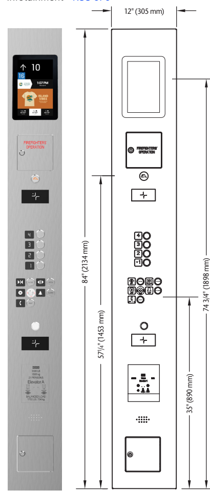
Car Operating Panel with KONE Infotainment + KSS 570
